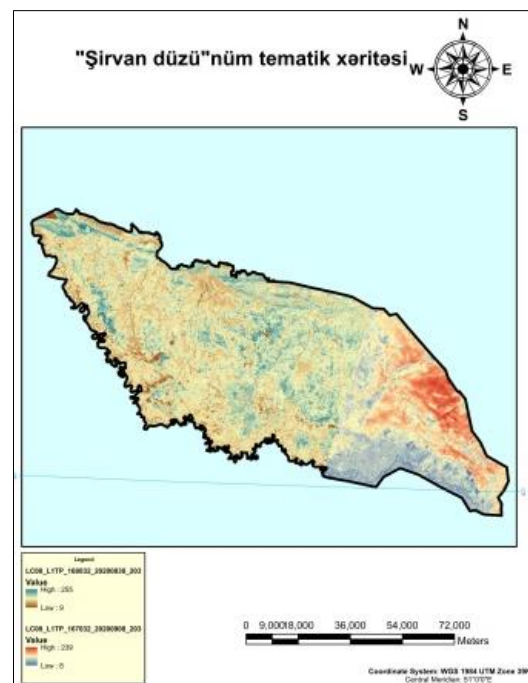
Fig 4: Thematic map of the length/slope (LS) factor
