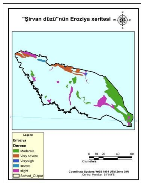
Fig 6: Soil erosion classification map.
