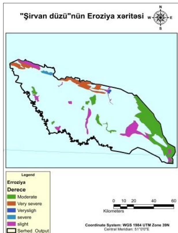
Fig 6: Soil erosion classification map.
